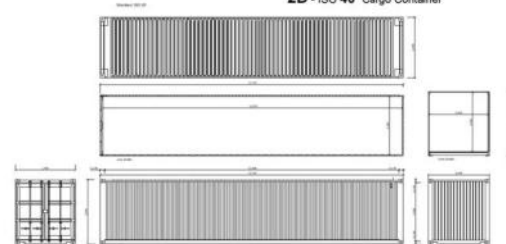
2D - ISO 40' Cargo Container
